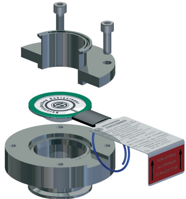
Reverse buckling bursting disc with membrane signal transmitter in bursting disc holder type BHS
