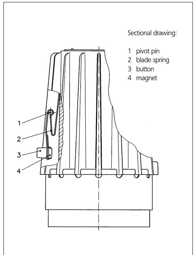
Lumiglas Time Delay Switch as optional feature for Ex as well as Non-Ex Lumiglas luminaires.
